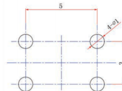
Hole Positions On The Circuit Board
