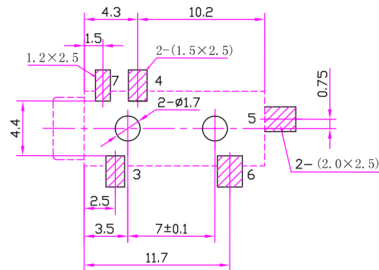
PCB Mounting Location Diagram
