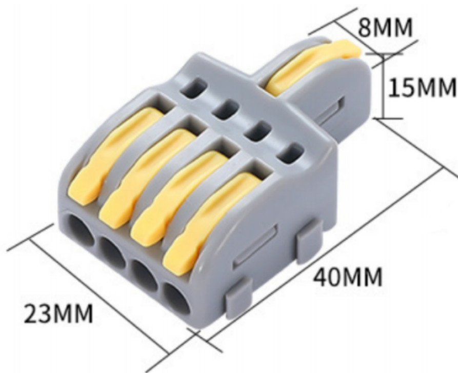
One-in four-out yellow terminal block
