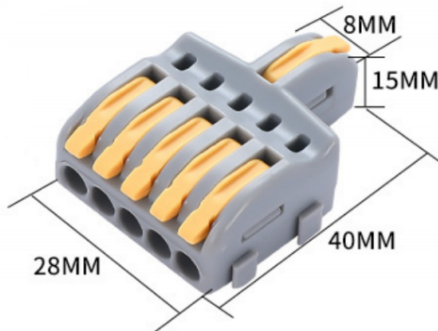
One-in five-out yellow terminal block
