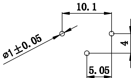
Mounting Dimensions
