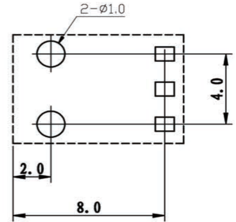
Schematic of PCB Installation Dimensions
