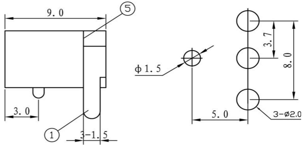
Schematic of PCB
