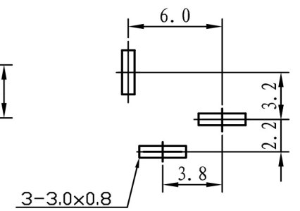
Schematic Diagram of Installation Dimension of Circuit Board
