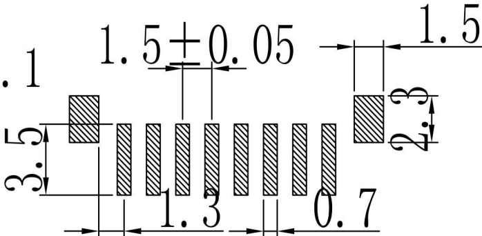
Printing Schematic of PCB(Tolerance ±0.05)
