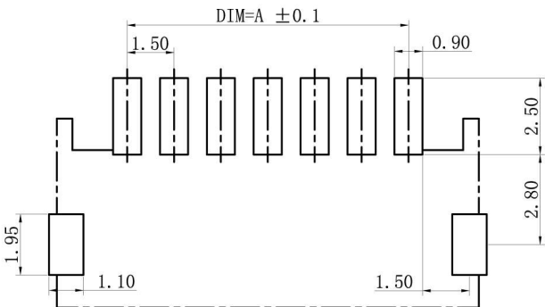
P. C. B LAYOUT REF
