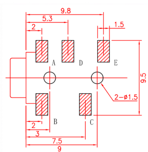
Schematic diagram of printed circuit board openings
