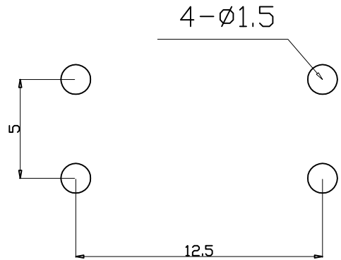
Mounting Dimensions
