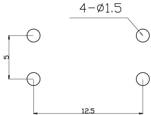
Mounting Dimensions
